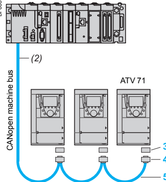
Example of CANopen diagram with SUB-D connector
