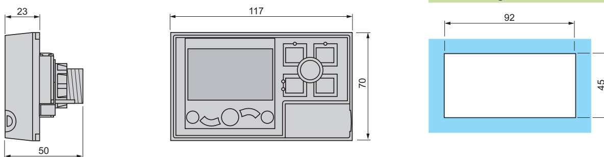
Panel mounting, cut-out
